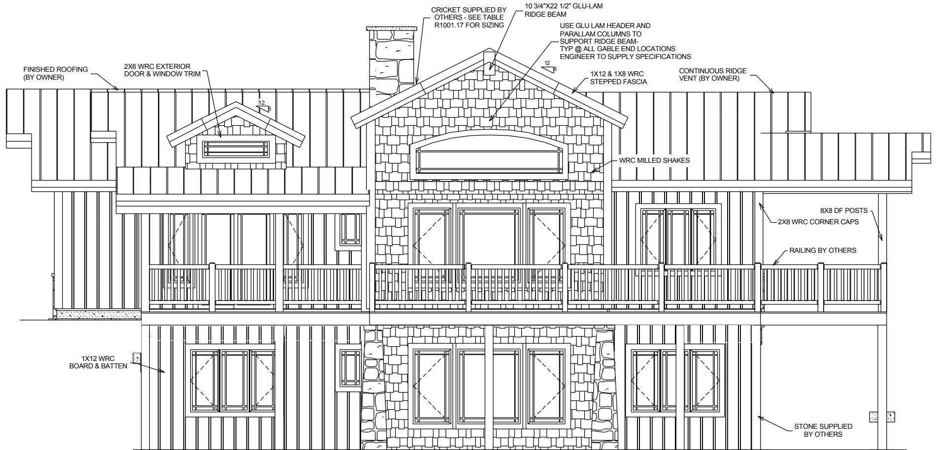
REAR ELEVATION
